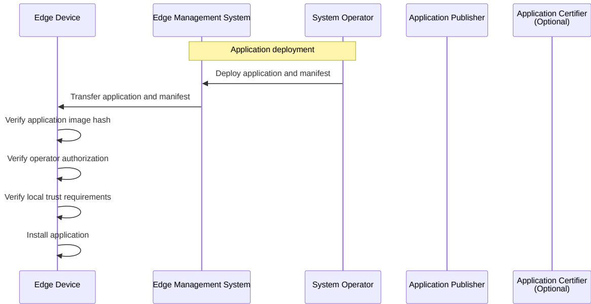
Figure 7.5: Sequence diagram showing application deployment
