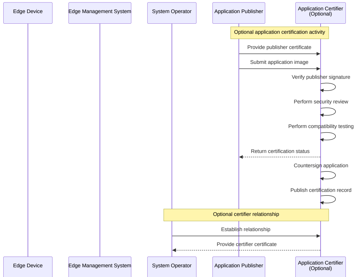
Figure 7.2: Sequence diagram showing optional application certification
