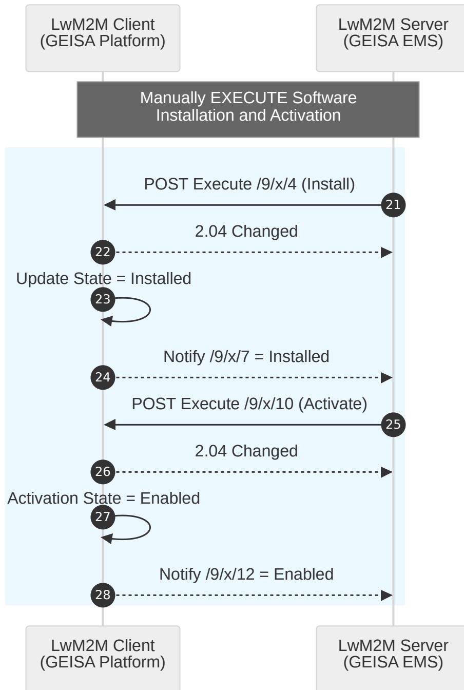
Figure 11.10: Edge App Install and Activate
