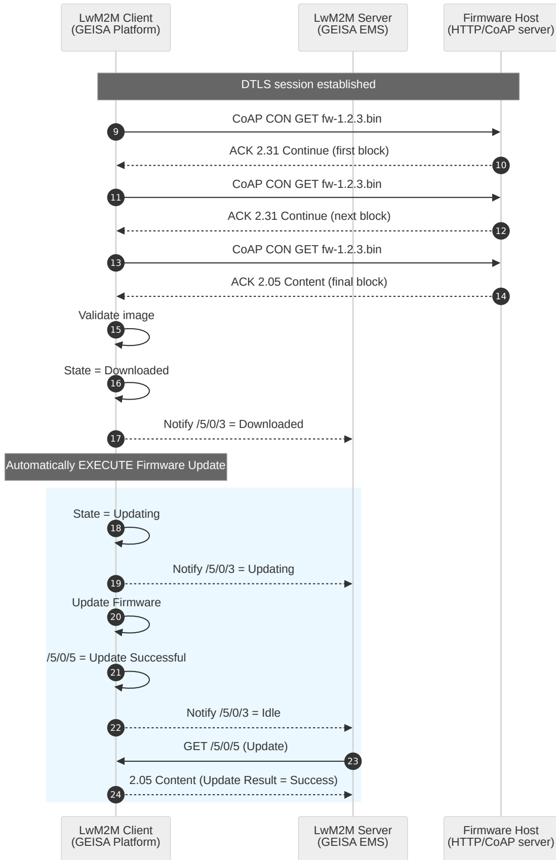
Figure 11.8: Firmware Over-the-Air Pull Automatic Download and Update
