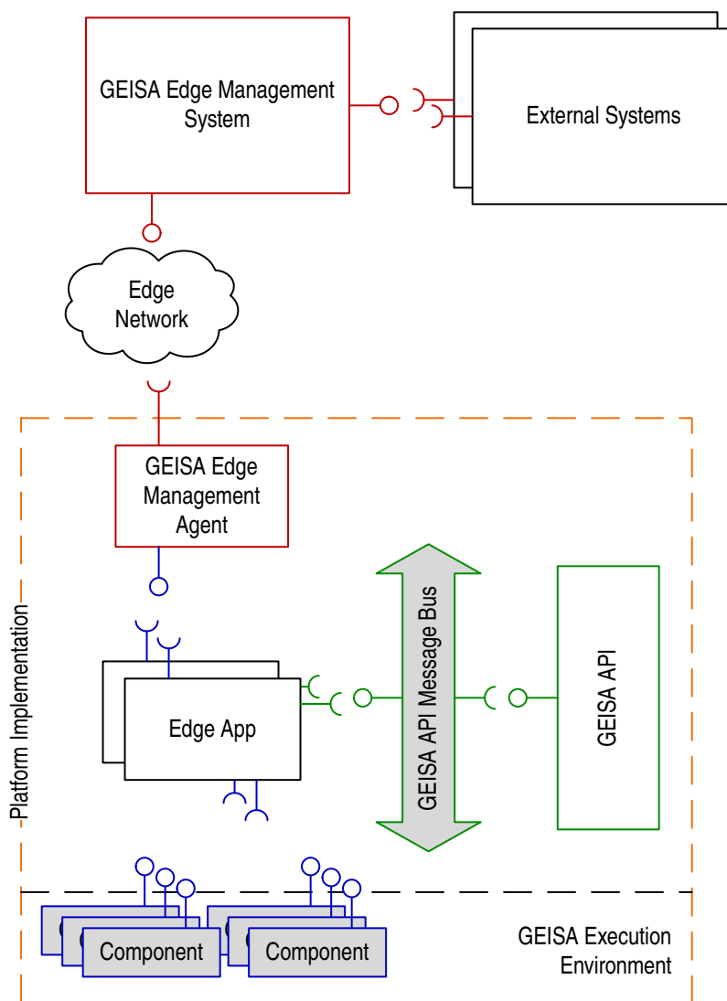
Figure 8.1: GEISA Architecture
