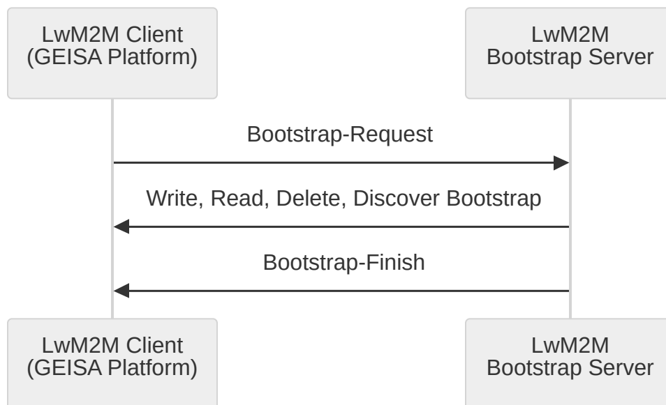
Figure 11.1: Client Bootstrap
