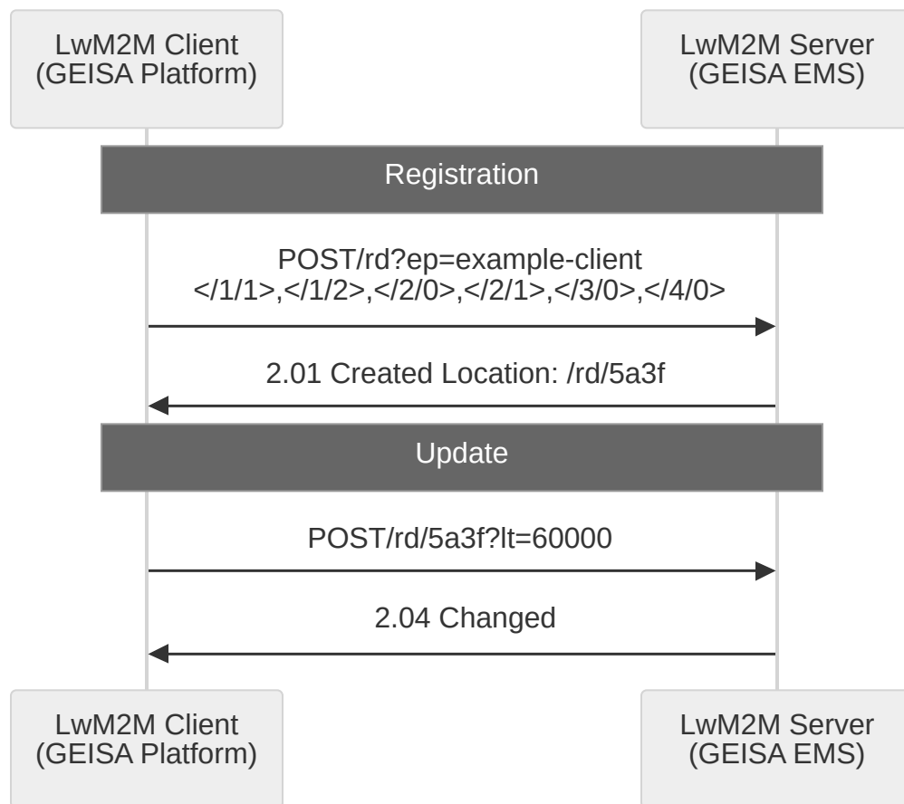
Figure 11.2: LWM2M Registration and Registration Update
