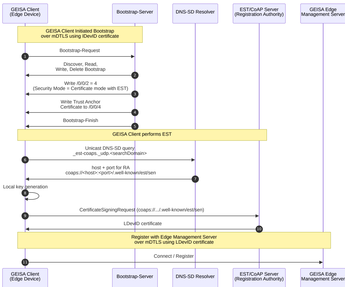
Figure 15.1: Enrollment over Secure Transport triggered by Client-Initiated Bootstrap
