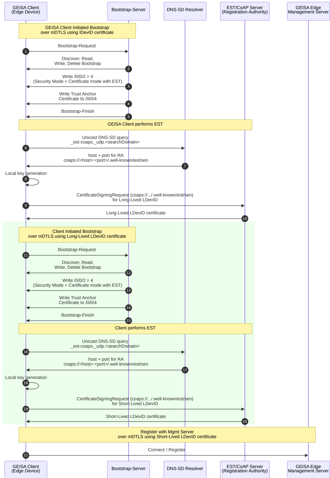
Figure 15.2: Enrollment over Secure Transport triggered by Client-Initiated Bootstrap with long-lived and short-lived LDevIDs
