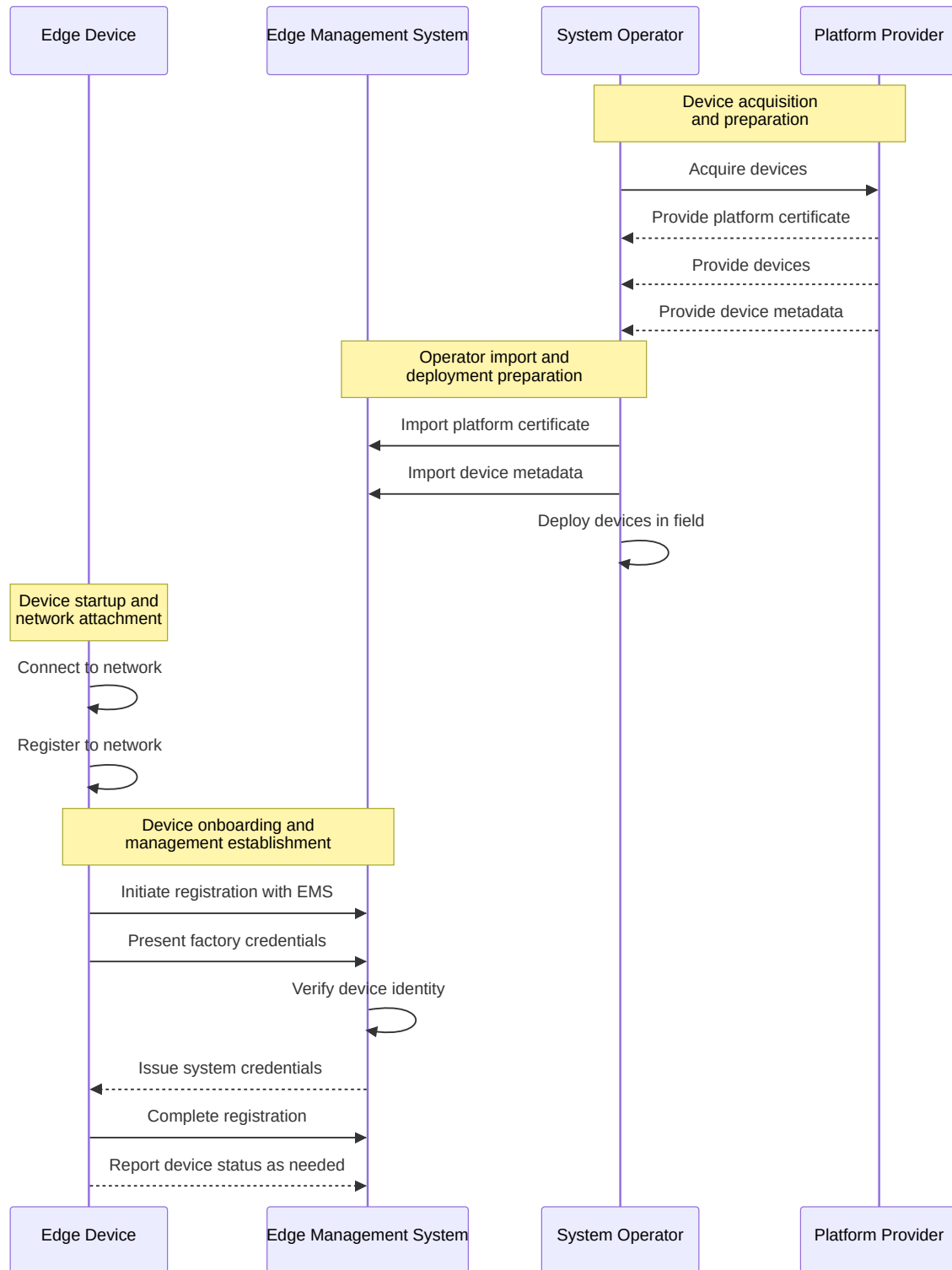
Figure 7.7: Sequence diagram showing device onboarding
