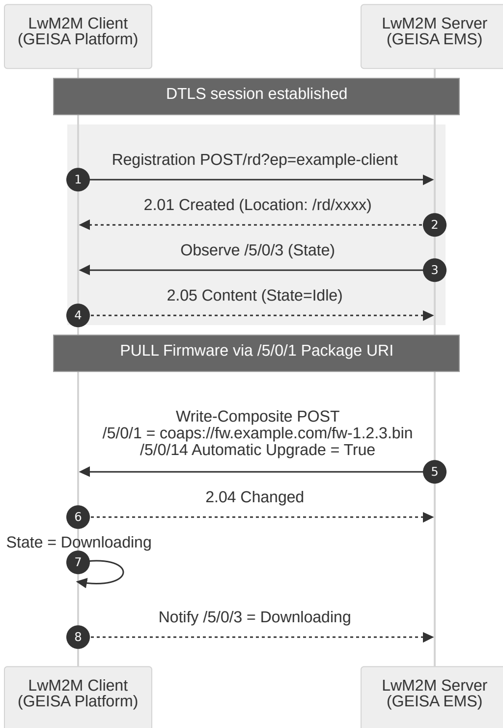
Figure 11.7: Firmware Over-the-Air Pull Image Initiate
