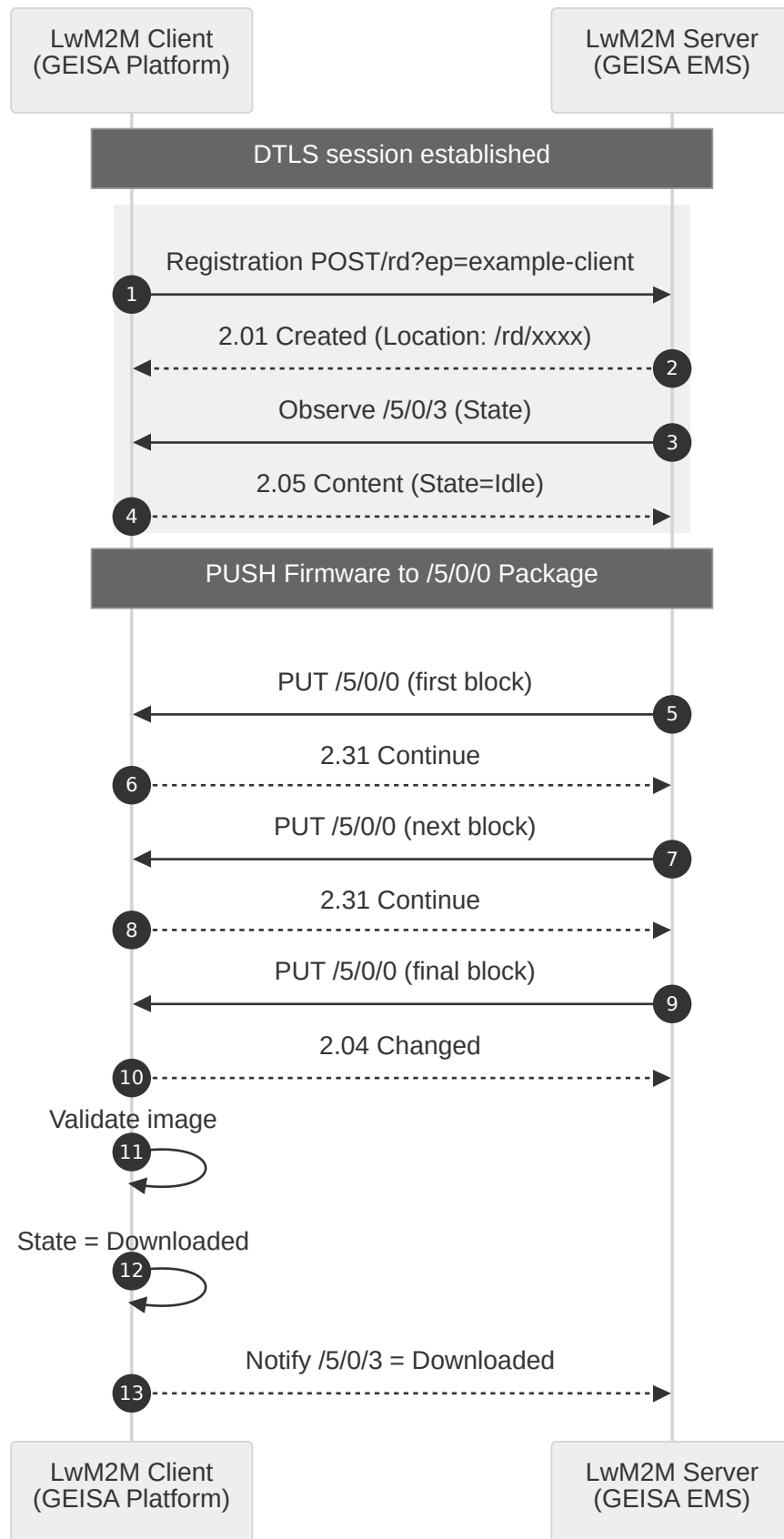
Figure 11.5: Firmware Over-the-Air Push Update
