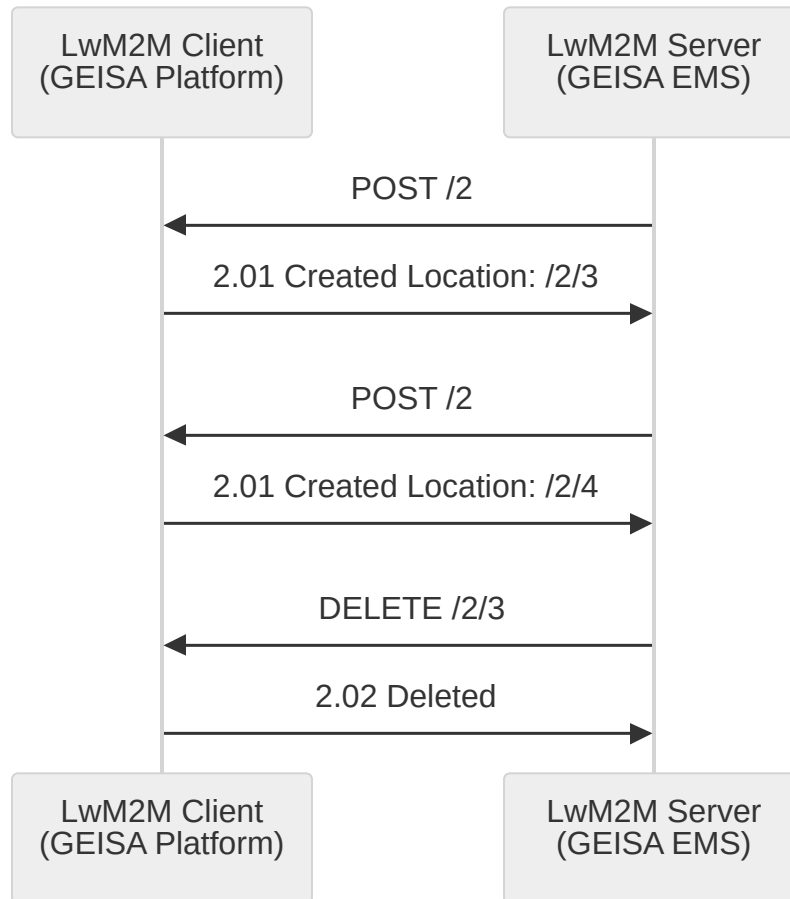
Figure 11.4: Object Creation and Deletion
