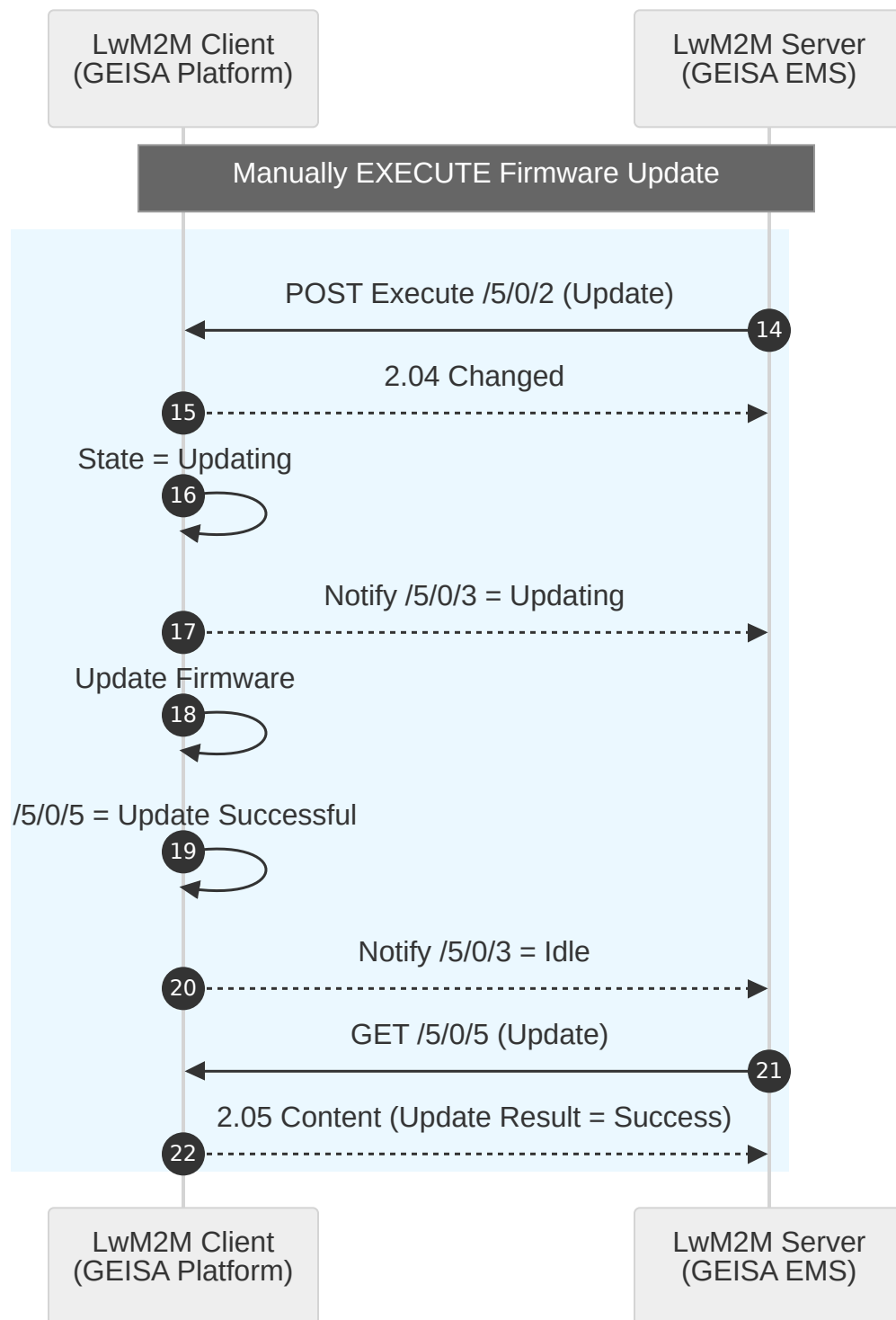
Figure 11.6: Firmware Over-the-Air Manual Activate
