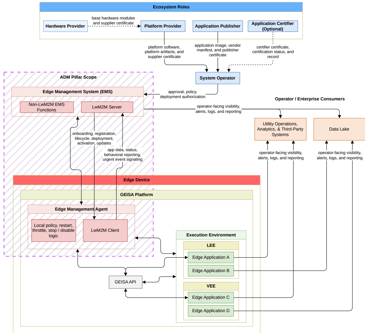
Figure 7.1: High-level GEISA operational context showing how principal roles and components relate end to end.
