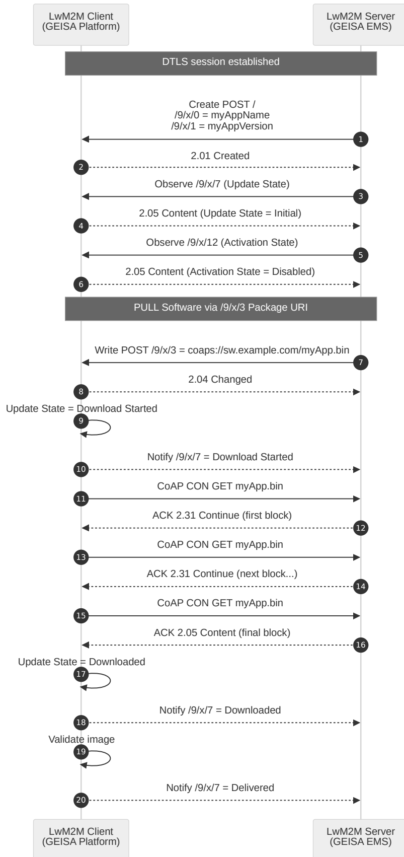
Figure 11.9: Edge App Image Pull
